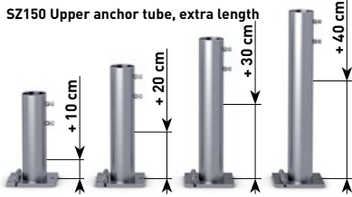
SZ150 Upper anchor tube, extra length
