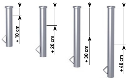
DMZ118 Lower anchor tube, extra length
